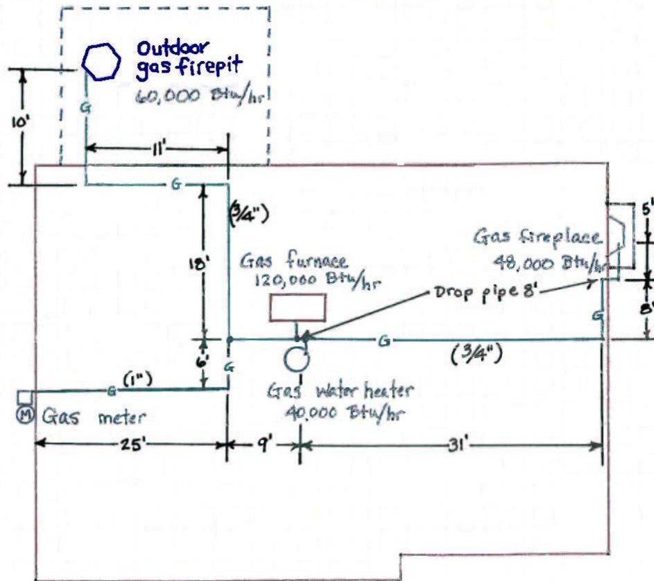
Example Drawing of Gas Piping Schematic
